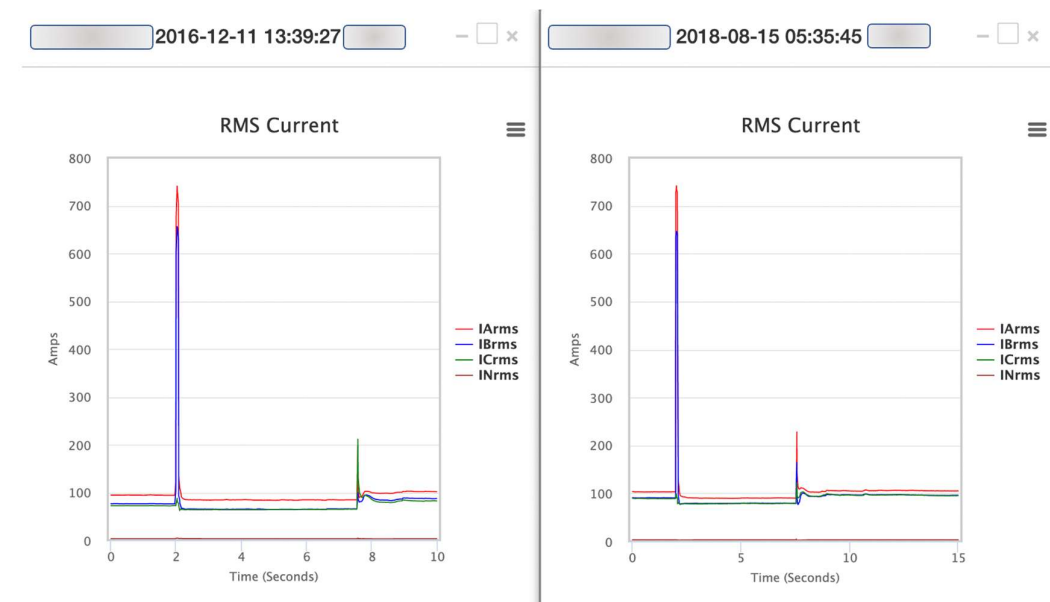
Figure 1: Two identical faults 20 months apart
