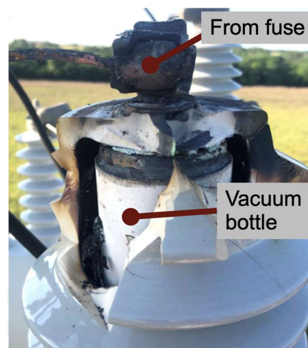
Figure 7: Damaged capacitor switch
