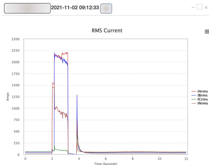
Figure 2: Initial fault, Case Study 1
