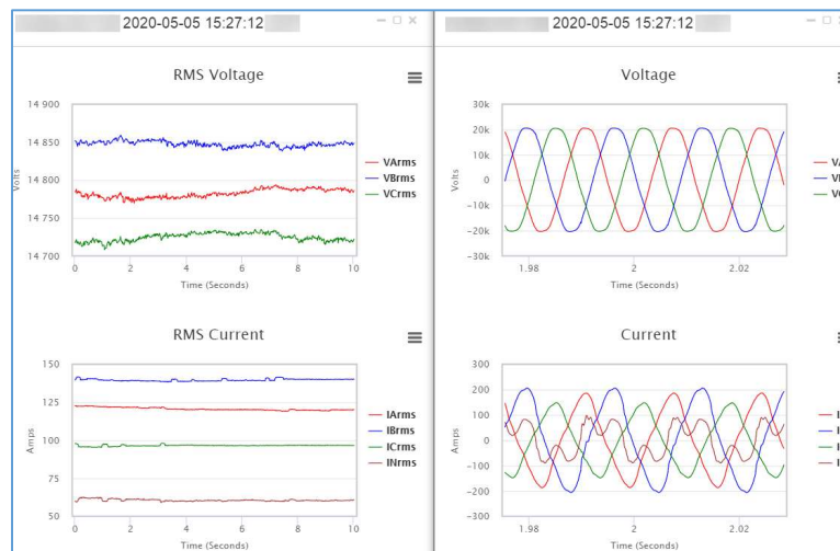
Figure 6: RMS and oscillography, capacitor arcing
